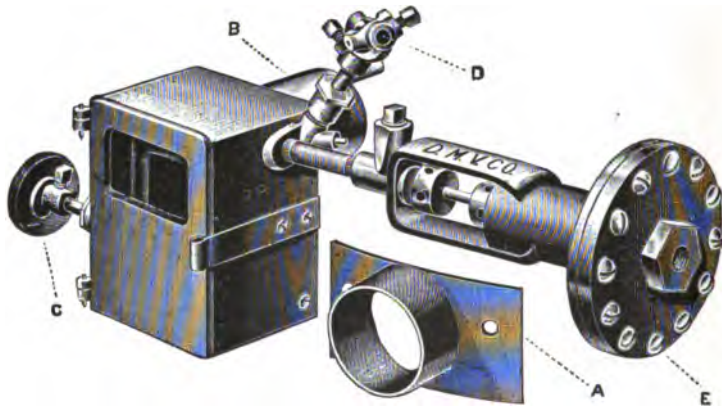
FIG. 220.—Starter Box and Diaphragm Regulator of the "Dayton" Burner. The parts are: A, segmental plate and collar at opening of the mixing tube; B, thimble on starter box containing supply pipe to the mixing tube and burner; C, starting valve; D, knuckle joint for connecting control valve to driver's seat; E, head piece of the diaphragm regulator.
